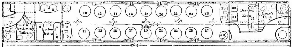
Fig. 190. Sectional Plan. PARLOR CAR, SANTA MARIA. (Interior view is shown in Fig. 117.)
